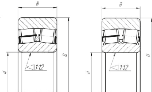
SPHERICAL ROLLER BEARINGS ON THE INNER RING WITH TAPERED BORE , TAPER 1:12 External design: K suffix
